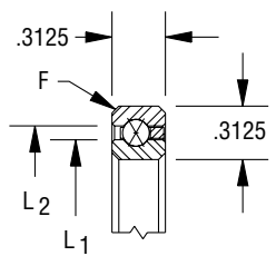
Snapover separator 5/32" balls
