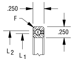
Snapover separator 1/8" balls
