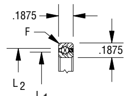
Snapover separator 3/32" balls
