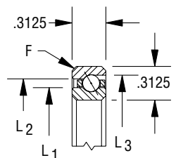
Circular pocket separator 5/32" balls
