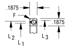
Circular pocket separator 3/32" balls
